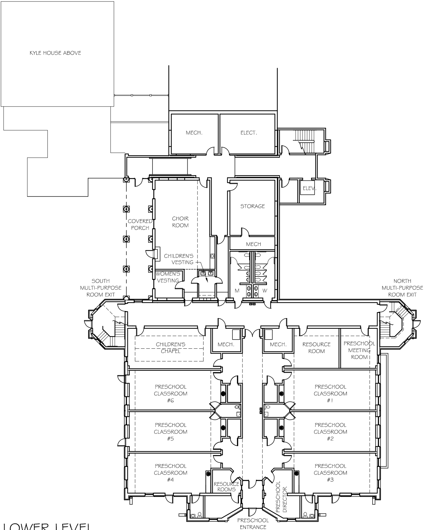
LOWER LEVEL FLOOR PLAN
